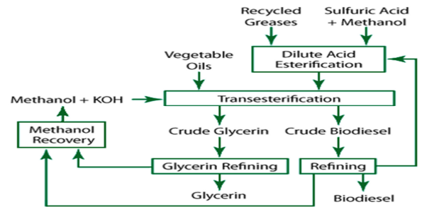
Figure 1 Schematic representation of biodiesel production.
